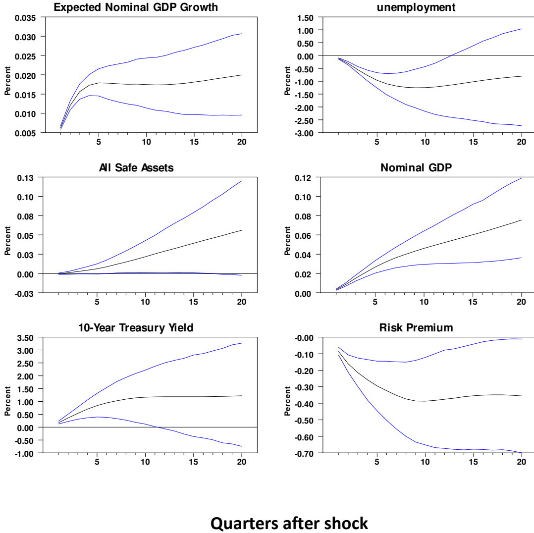
Figure 2: Response to Typical Shock to Expected NGDP Growth (1968:Q4 – 2011:Q4)
