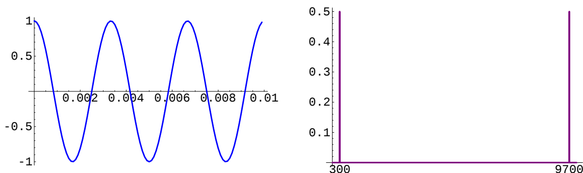
Figure 3: Sampled points for a 300 Hz tone over 0.01 seconds, and the Fourier transform of the entire second of sampled points.
